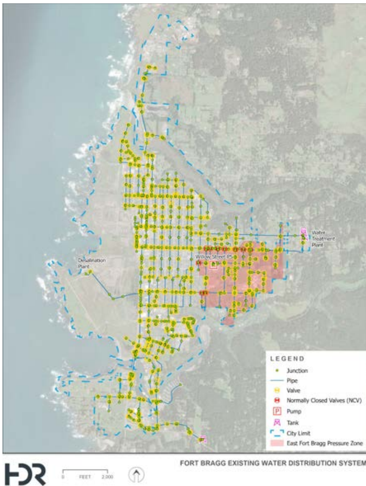
Figure 14 – Fort Bragg Existing Water Distribution System
