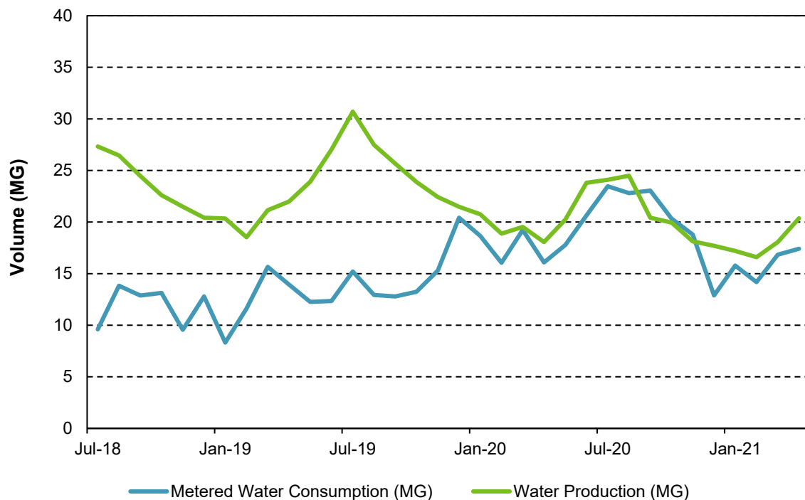
Figure 8 – Water Production Versus Metered Water Consumption Comparison
