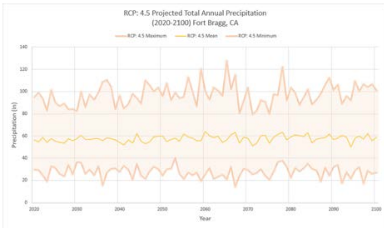
Figure 11 – Projected Total Annual Precipitation for Fort Bragg Based on Climate Scenario RCP 4.5.
