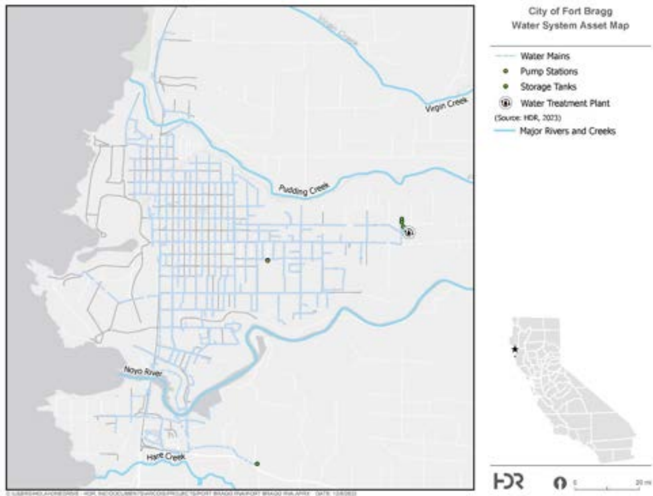
Figure 27 – Water Distribution Assets Map (Source: HDR GIS based on Fort Bragg database)
